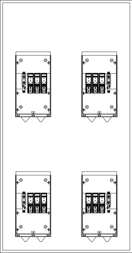
DETALLE 4 C.G.P.
