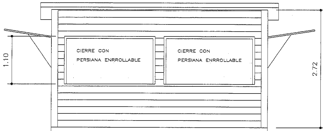
ALZADO PRINCIPAL
